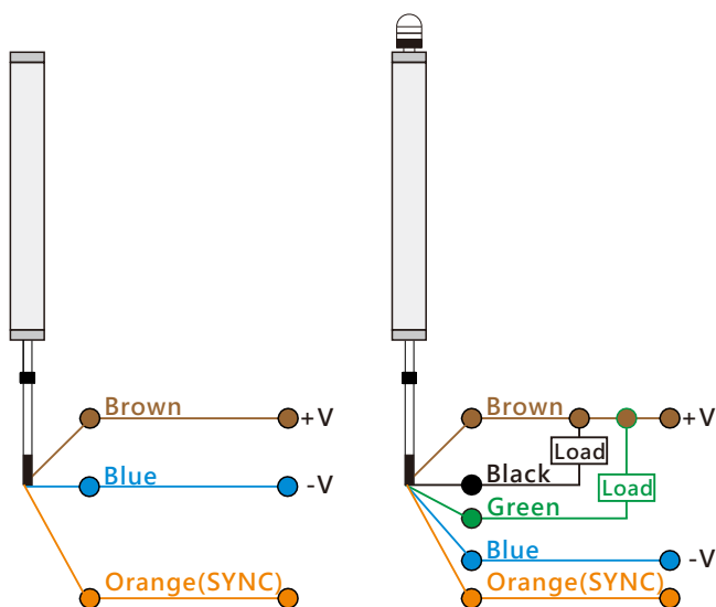
NPN NO&NC Type Direct connecting method
