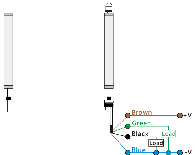
PNP NO&NC Type Y-connecting method
