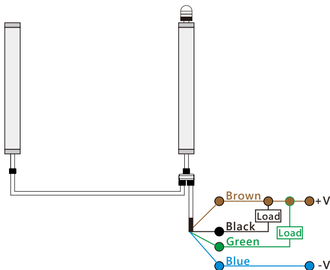
NPN NO&NC Type Y-connecting method
