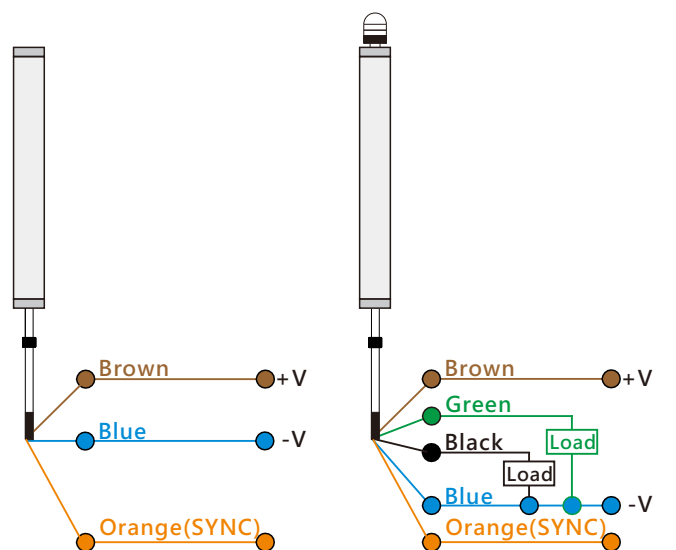
PNP NO&NC Type Direct connecting method
